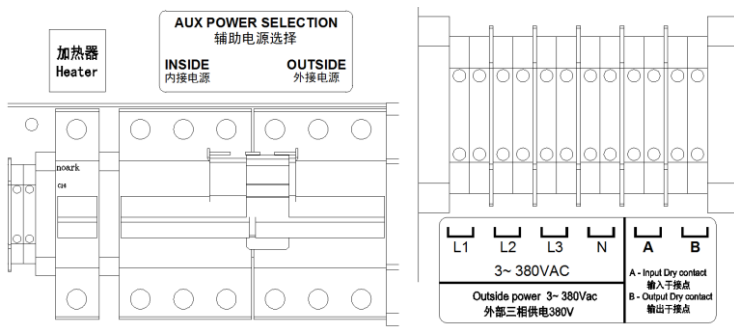
图 3-19 CPS SCA630/500kW 带加热器外接电源和干接点接线
